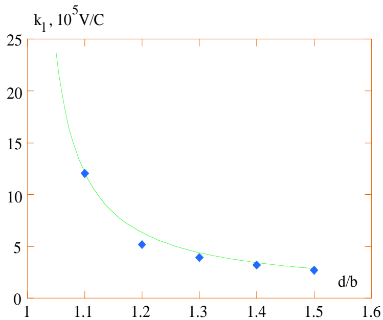
Fig. 3 - Dependence of the loss factor on the ratio of the pipe radii.
