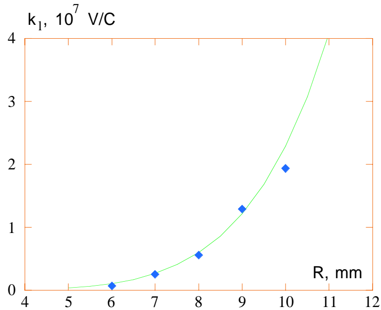
Fig. 2 - Dependence of the loss factor on the hole radius
