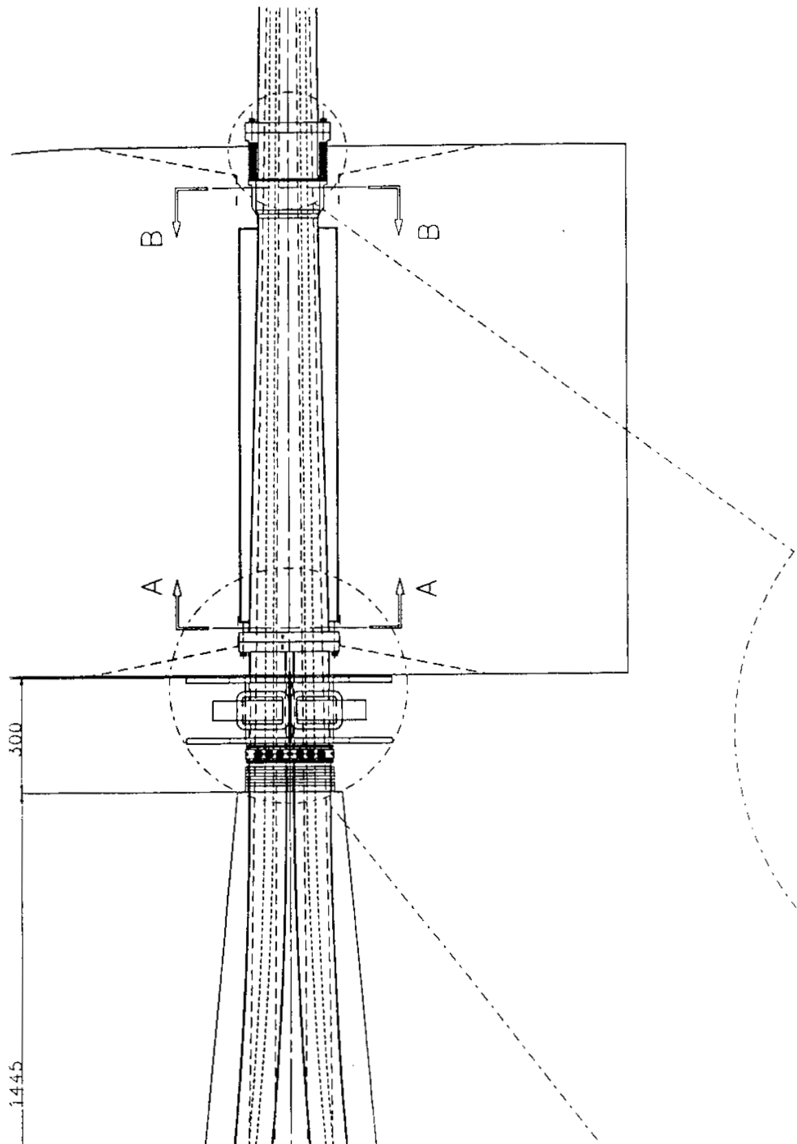
Fig. 15 - Intersection of two DAΦNE main rings.
