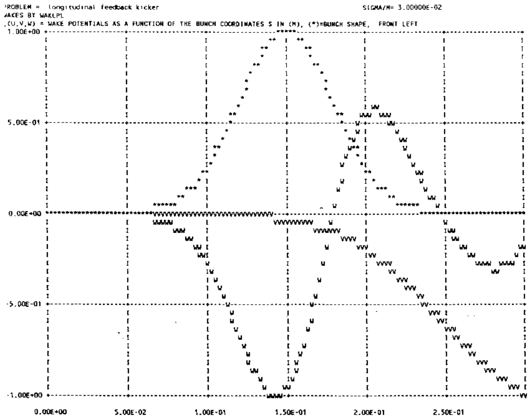
Fig. 13 - Normalized wake-function for the longitudinal feedback kicker (w).
