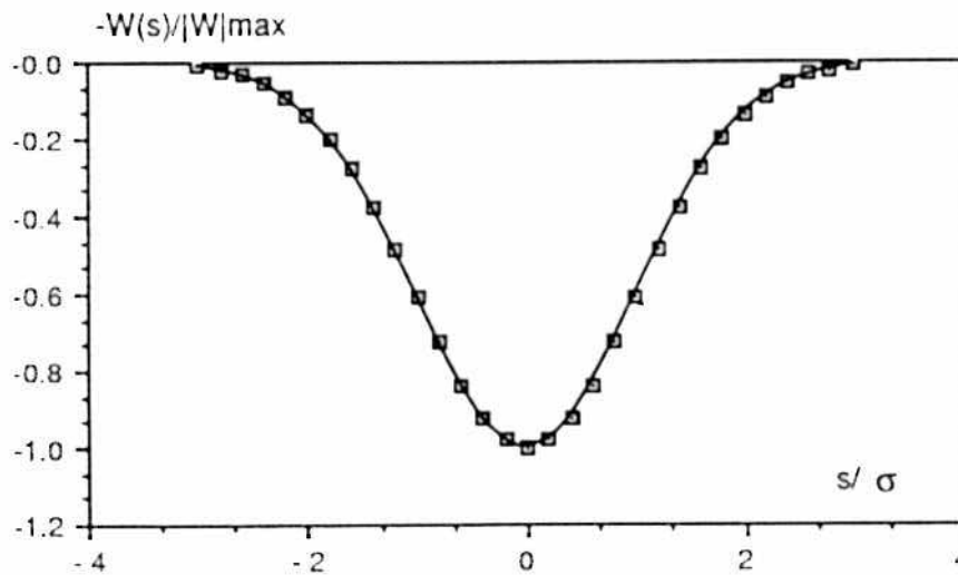
Fig. 2 - Normalized wake-function corresponding to the resistive impedance Z(\omega) = R .
