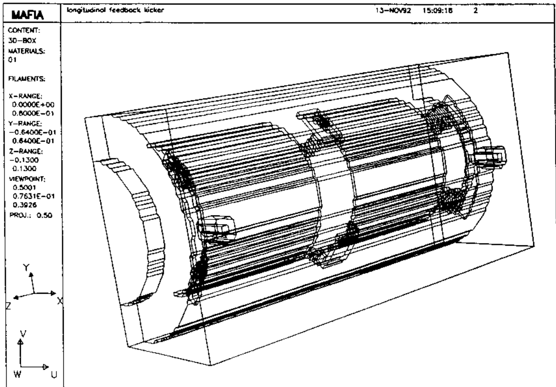
Fig. 12 - Longitudinal feedback kicker (half a structure).
