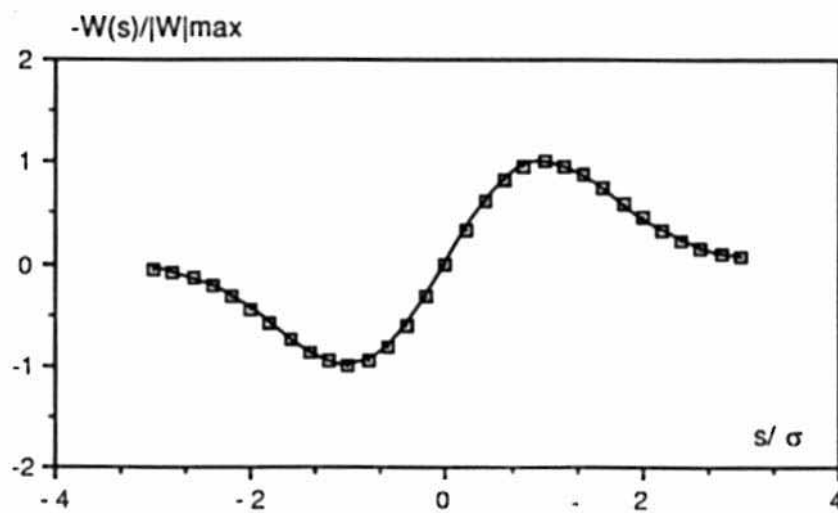
Fig. 1 - Normalized wake-function corresponding to the inductive impedance Z(\omega) = -i\omega L .
