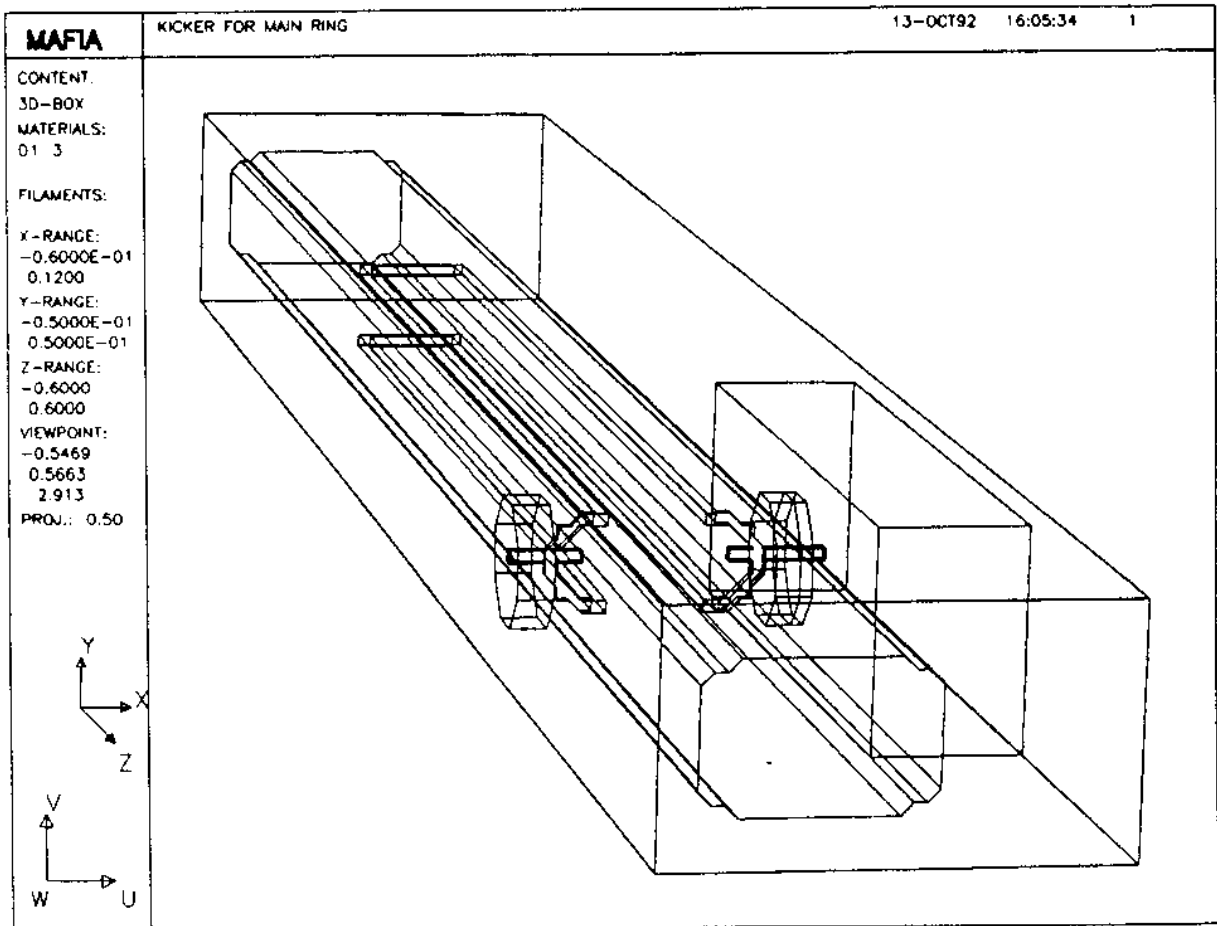
Fig. 9 - Injection kicker .
