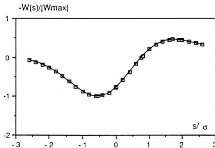
Fig. 3 - Normalized wake-function corresponding to the impedance Z(\omega) = (1 - i) B \sqrt{\omega} .
