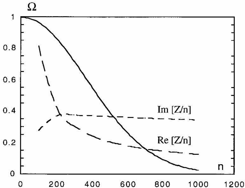
Fig. 23 - Imaginary and real part of DAΦNE main ring impedance with superimposed bunch spectrum (solid line).
