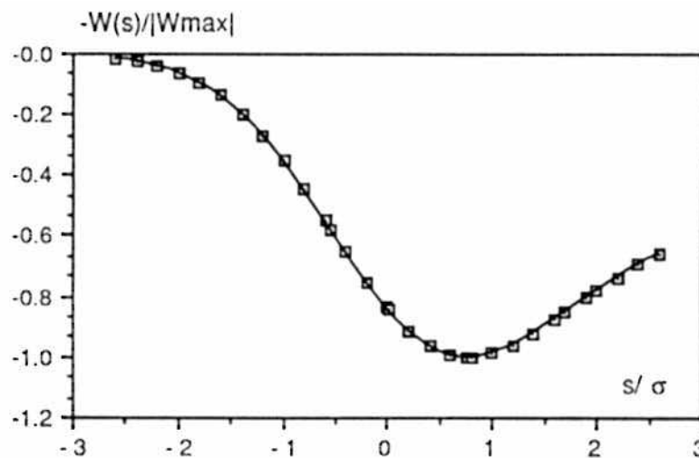
Fig. 4- Normalized wake-function corresponding to the impedance Z(\omega) = \frac{(1+i)Z_c}{\omega} .
