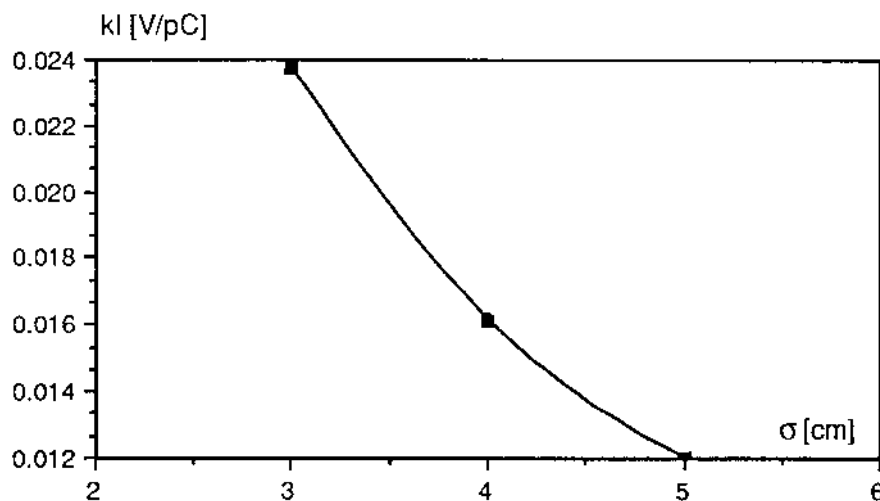
Fig. 10 - Fit of the longitudinal loss factor for the injection kicker; numerical and analytic curves coincide.
