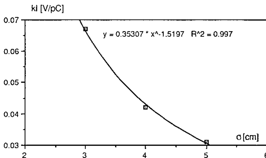
Fig. 14 - Dependence of the longitudinal loss factor on the bunch length for the longitudinal feedback kicker.
