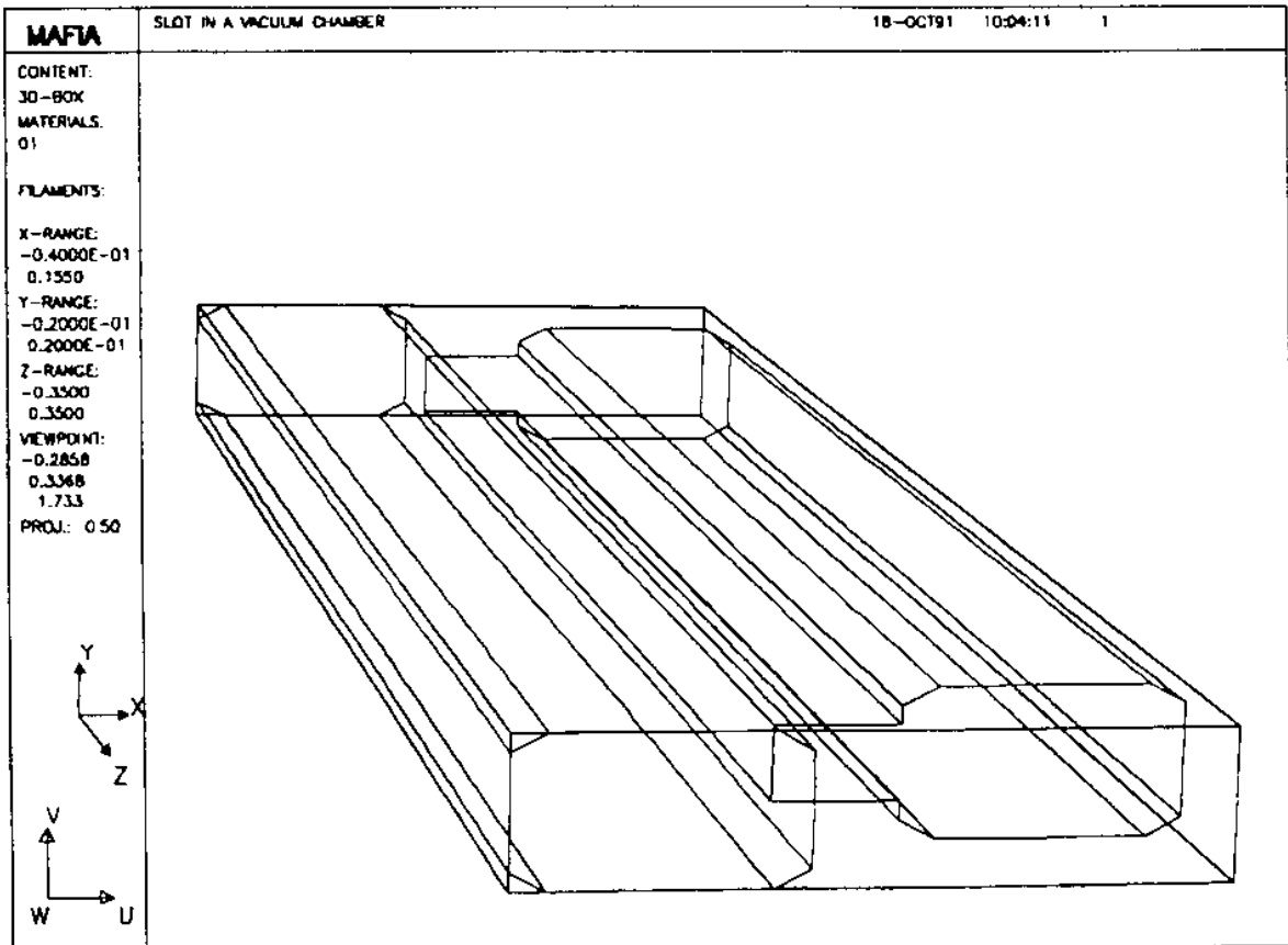
Fig. 19 - Slot between antechamber and regular vacuum chamber .
