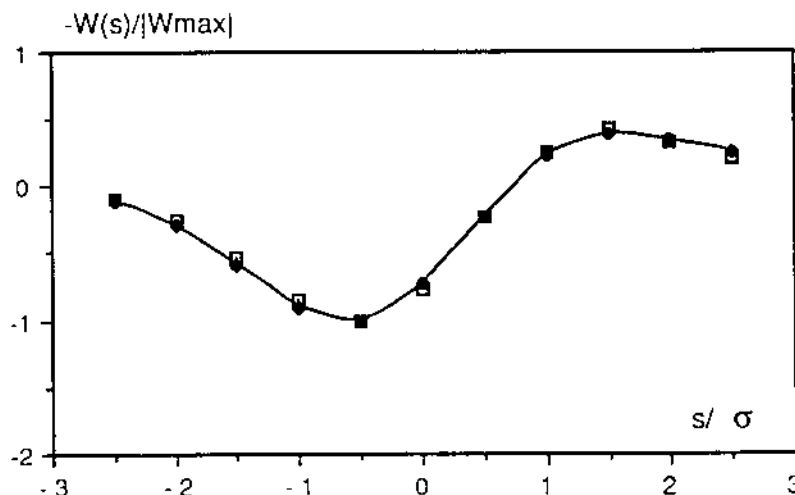
Fig. 11 - Fit of the normalized wake-function for the injection kicker; full dots: MAFIA code results; open squares: wake-function corresponding to the impedance model (1).
