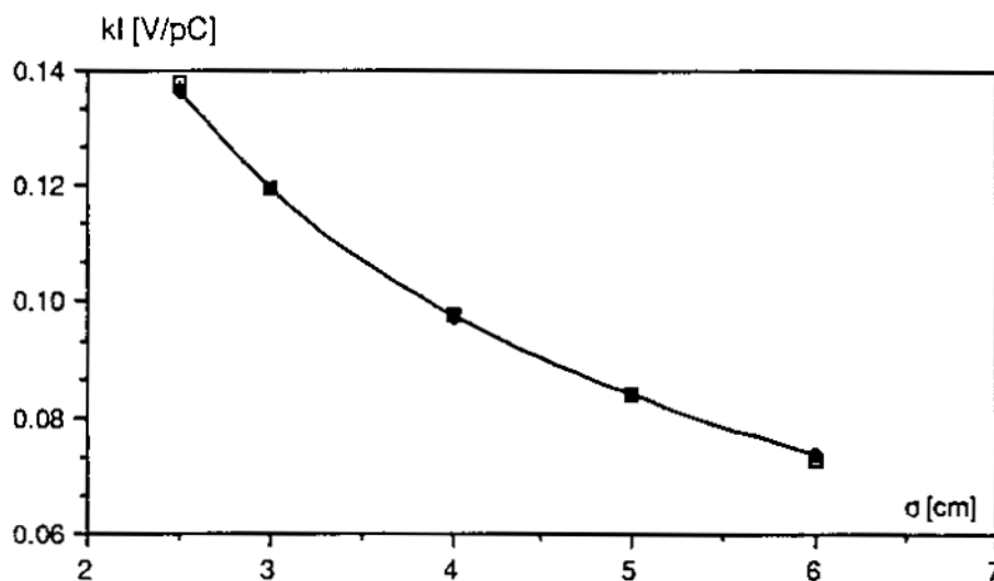
Fig. 7 - Fit of dependence k_e(\sigma) with the broad-band model given by eq.(1). Analytical and numerical curves coincide.
